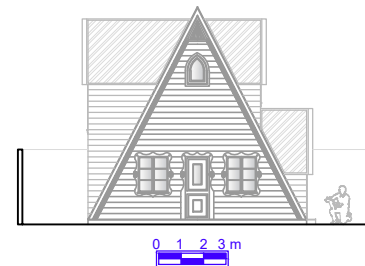
Elevation 03
